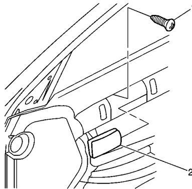
Figure 1 Removing Bezel
